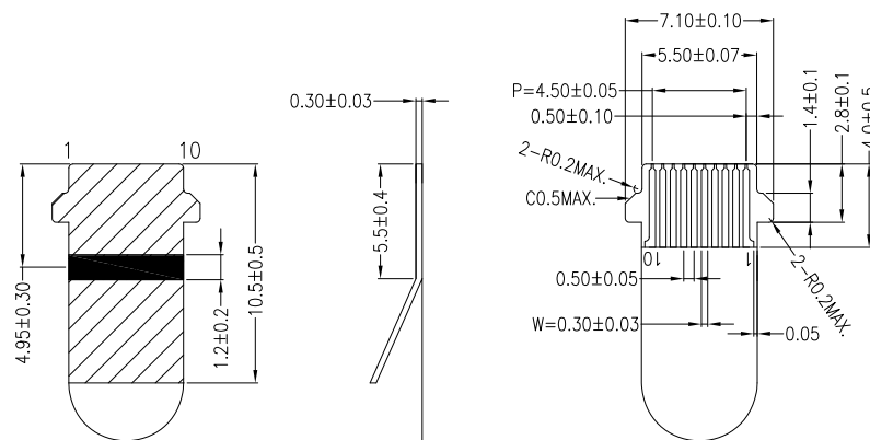
DETAIL A (SCALE 5:1)
